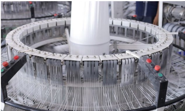
Circular Weaving Machine.
